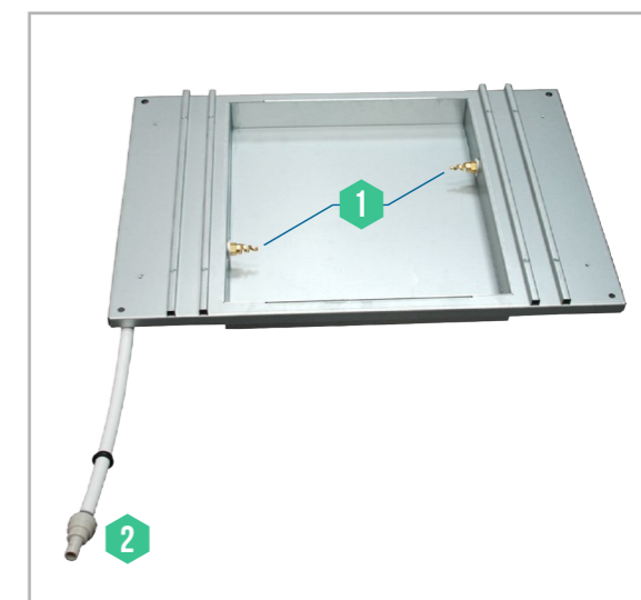
01 Wash nozzles
